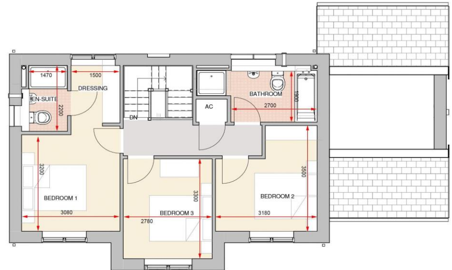
First Floor 1 : 50
